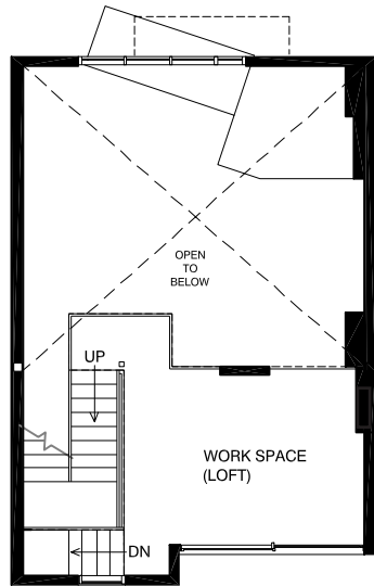
MEZZANINE PLAN
