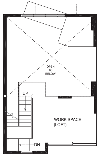
MEZZANINE PLAN
