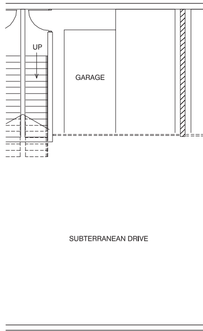
GARAGE LEVEL PLAN
